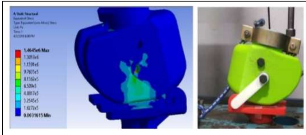
Figure 2. FEA analysis of prosthetic knee joint and experimental setup
